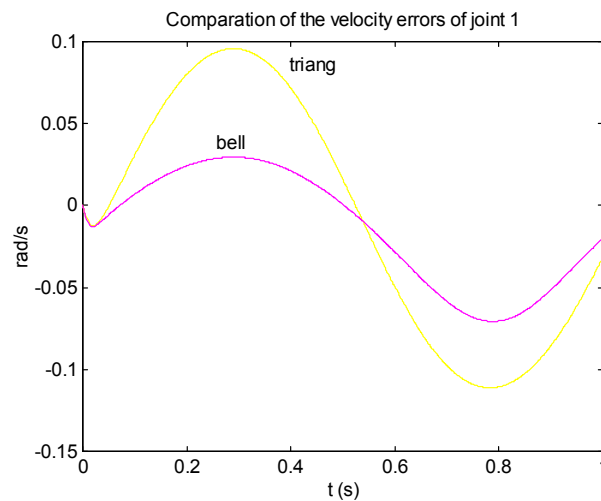
Figure 6. Comparison of the velocity errors on joint 1.
