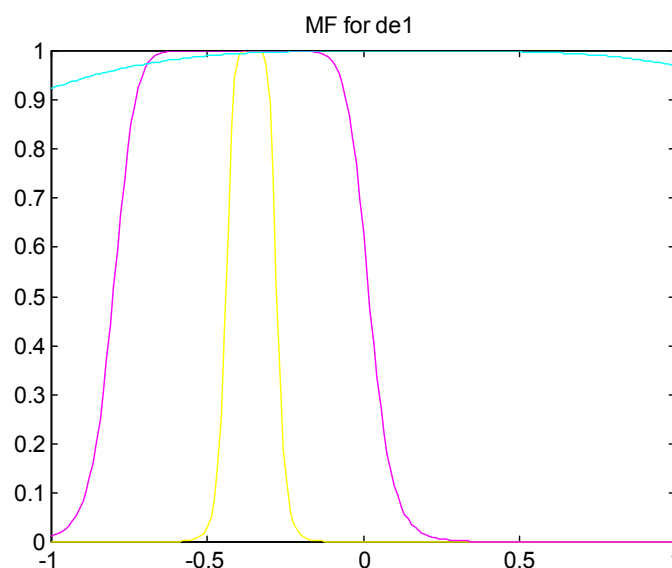
Figure 3. Optimized bell membership functions for de_1 .
