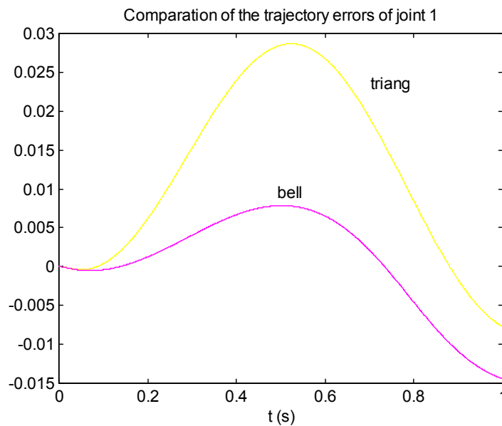
Figure 5. Comparison of the trajectory errors on joint 1.
