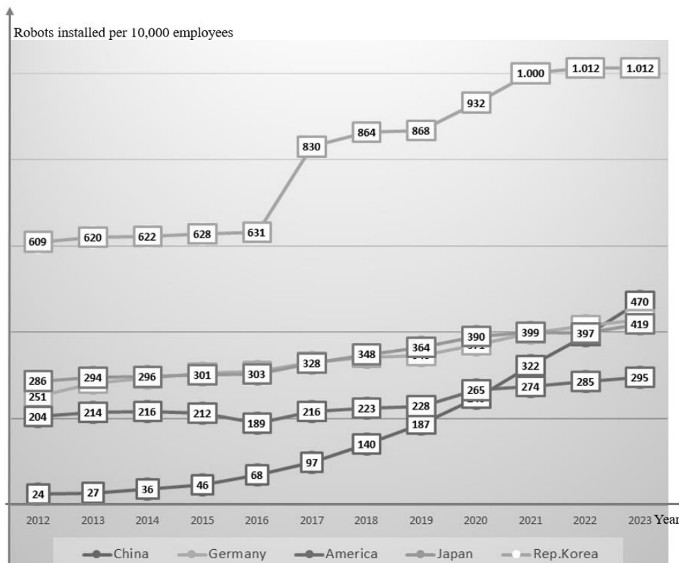
Figure 15. trend of industrial robot implementation per 10 000 employees in Japan, South Korea, Germany, the United States, and China, 2012-2023.
