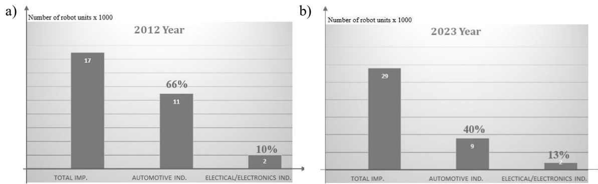
Figure 10. Implementation of industrial robots in the automotive and electrical/electronics industries in Germany in 2012 and 2023.
