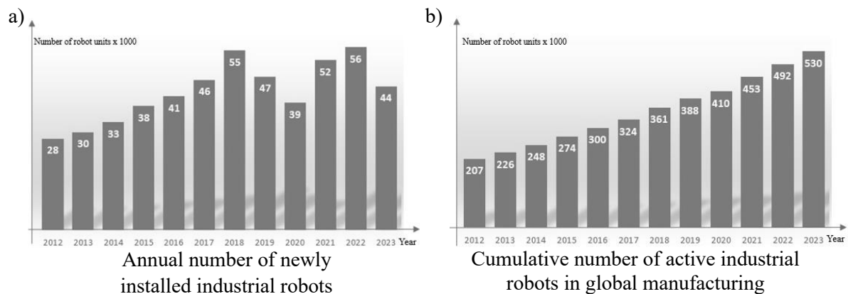
Figure 11. Trend in annual installations and total deployment of industrial robots in the United States, 2012-2023.
